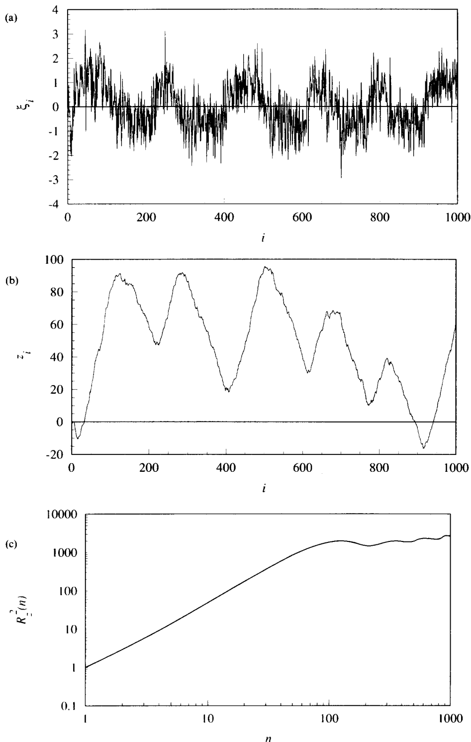
Figure 2. Representation of the fundamental quantities involved in the diffusional analysis. The time series refers to density fluctuations in intermittent regime, j_L = 2.07 m/s, j_G = 2.58 m/s recorded by the \gamma -densitometer. (a) Snapshot of the density time-series \xi_i vs i . \Delta t = 10^{-3} s; (b) z_i vs i ; (c) R_z^2(n) vs n .
