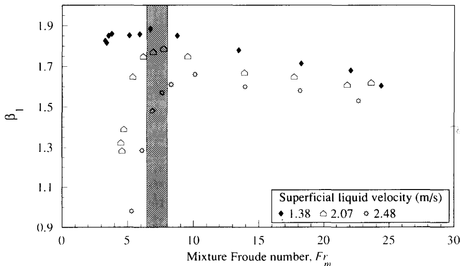
Figure 3. Behavior of the scaling exponent \beta_1 , see [6], in slug regime vs Froude number for different values of the liquid velocity j_L . The local maximum in \beta_1 is an indicator of high coherent fluctuations.
