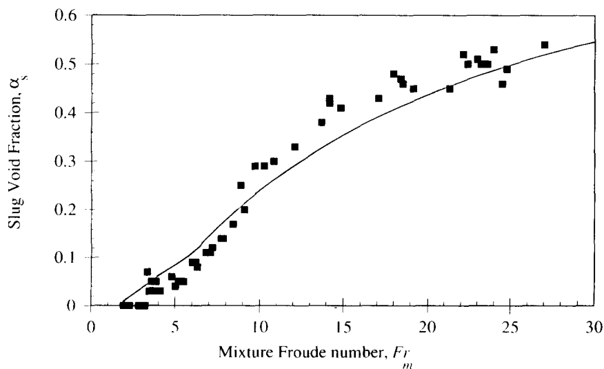
Figure 10. Average volumetric gas fraction in the liquid slug vs Froude number. Experimental data obtained in this work. Theoretical prediction obtained using C_1 = 13.33 and C_2 = 114.5 . For the region Fr_m > 6 , the values S_D = 1 , C_0 = 1.2 and V_0 = 0.0 m/s were used. For the region Fr_m < 6 , the values S_D = C_0 = 1.109 , V_0 = 0.298 m/s were used.
