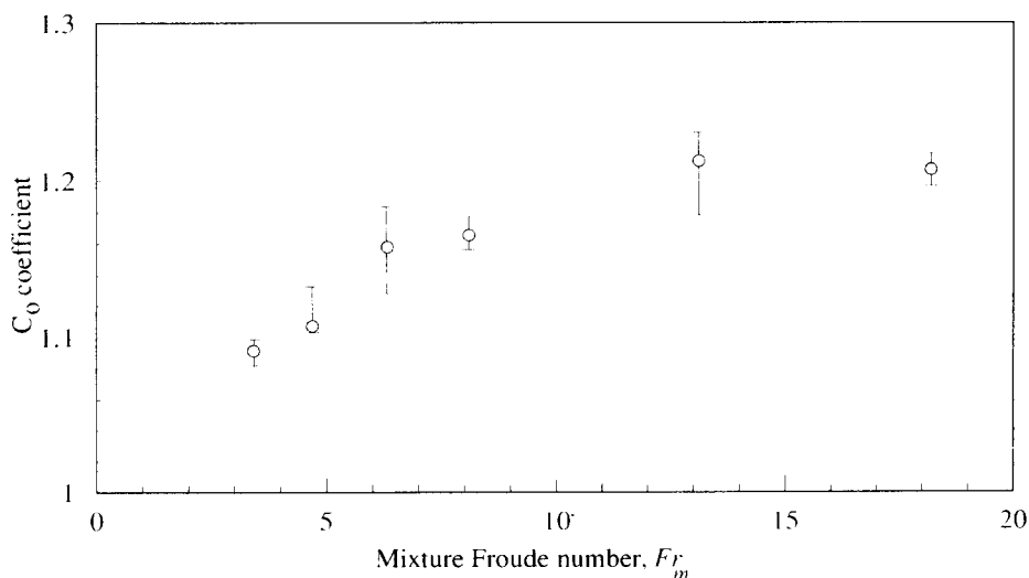
Figure 5. Measured bubble velocity and C_0 vs Froude number. Present experiments.
