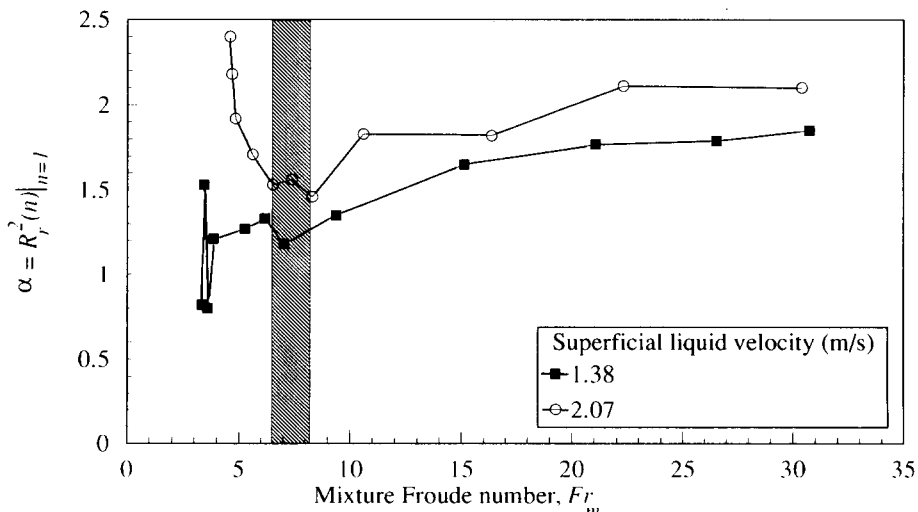
Figure 4. \alpha = R_r^2(1) vs Froude number in intermittent flow. The local minimum in \alpha indicates a lower intensity of stochastic fluctuations.
