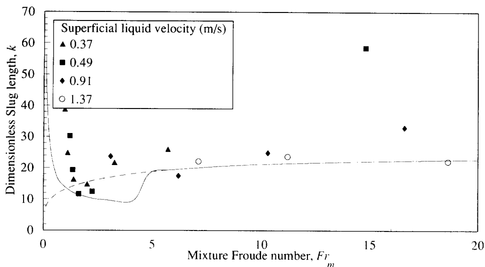
Figure 7. Average slug length vs Froude number. Comparison of the model suggested by Dukler et al. (1985) (dashed line), the present model (continuous line), and the experimental data of Nicholson et al. (1978).
