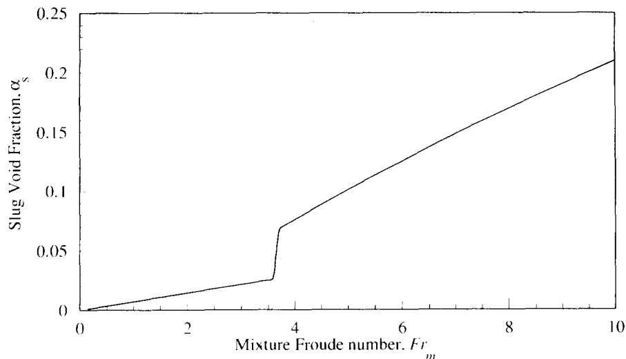
Figure 9. Average volumetric gas fraction in the liquid slug vs Froude number. Relation suggested by Andreussi & Bendiksen (1989)—air–water system d = 5 cm, horizontal pipe.
