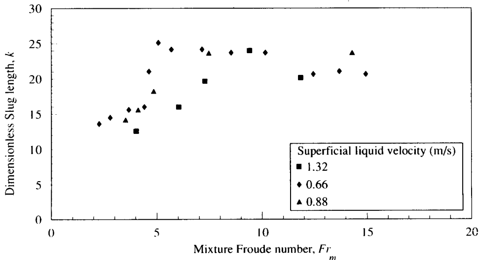
Figure 6. Average slug length vs Froude number. Data of Dukler & Hubbard (1975).
