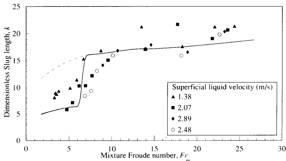
Figure 8. Average slug length vs Froude number. Comparison of the model suggested by Dukler et al. (1985) (dashed line), the present model (continuous line), and our experimental data.
